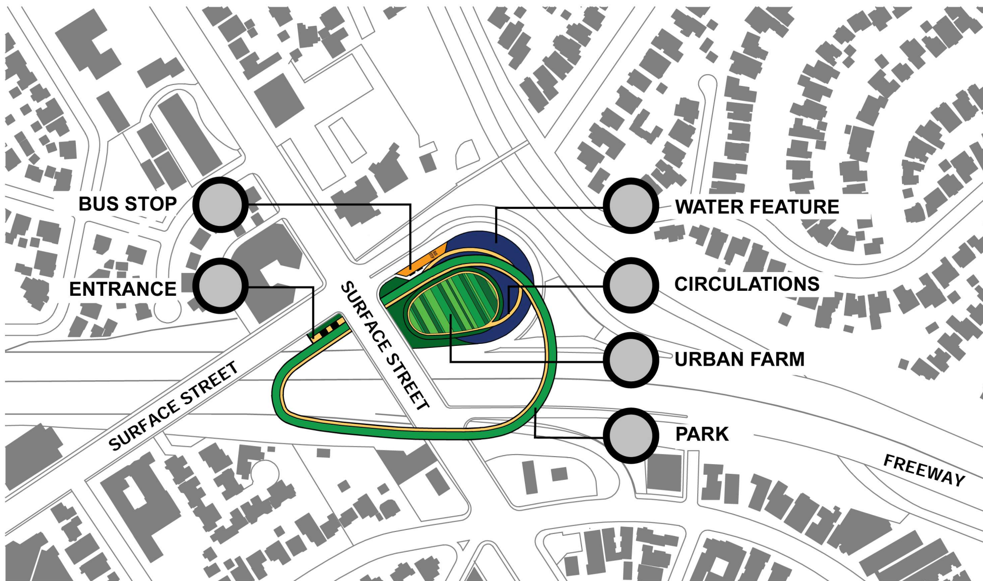
SITE PLAN
